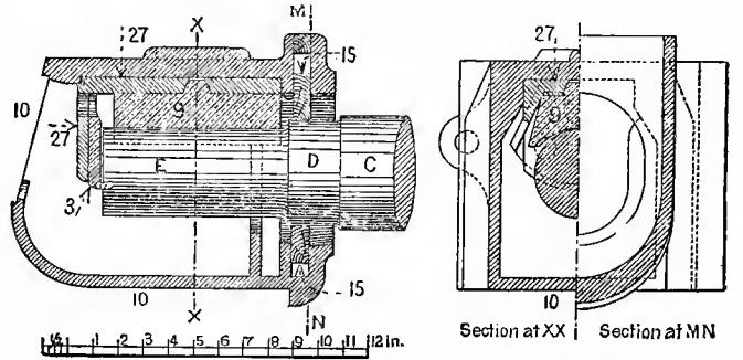
Fig. 5133. Section. Fig. 5134. BISSEL'S STOP-KEY JOURNAL BEARINGS FOR COLLARLESS JOURNALS.
